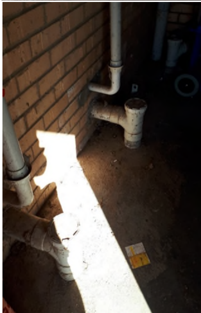
MOLONG RECREATION GROUND TOILET BLOCK – MAINTENANCE ROOM
